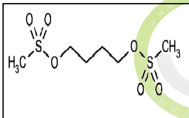
Figure 2: Structure of Busulfan
