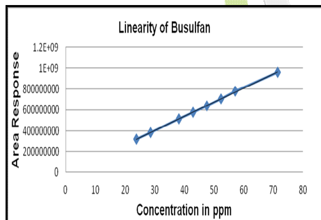
Figure 3: Linearity of Busulfan
